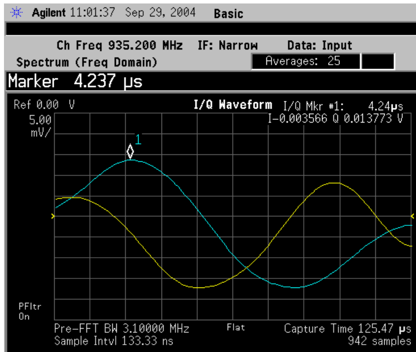
Figure 2-3 Spectrum (Time Domain) Measurement - I/Q Waveform Result
