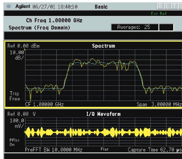
Figure 3-2 Spectrum Measurement - Spectrum and I/Q Waveform (Default View)
