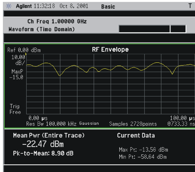
Figure 3-3 Waveform Measurement - RF Envelope (Default View)
