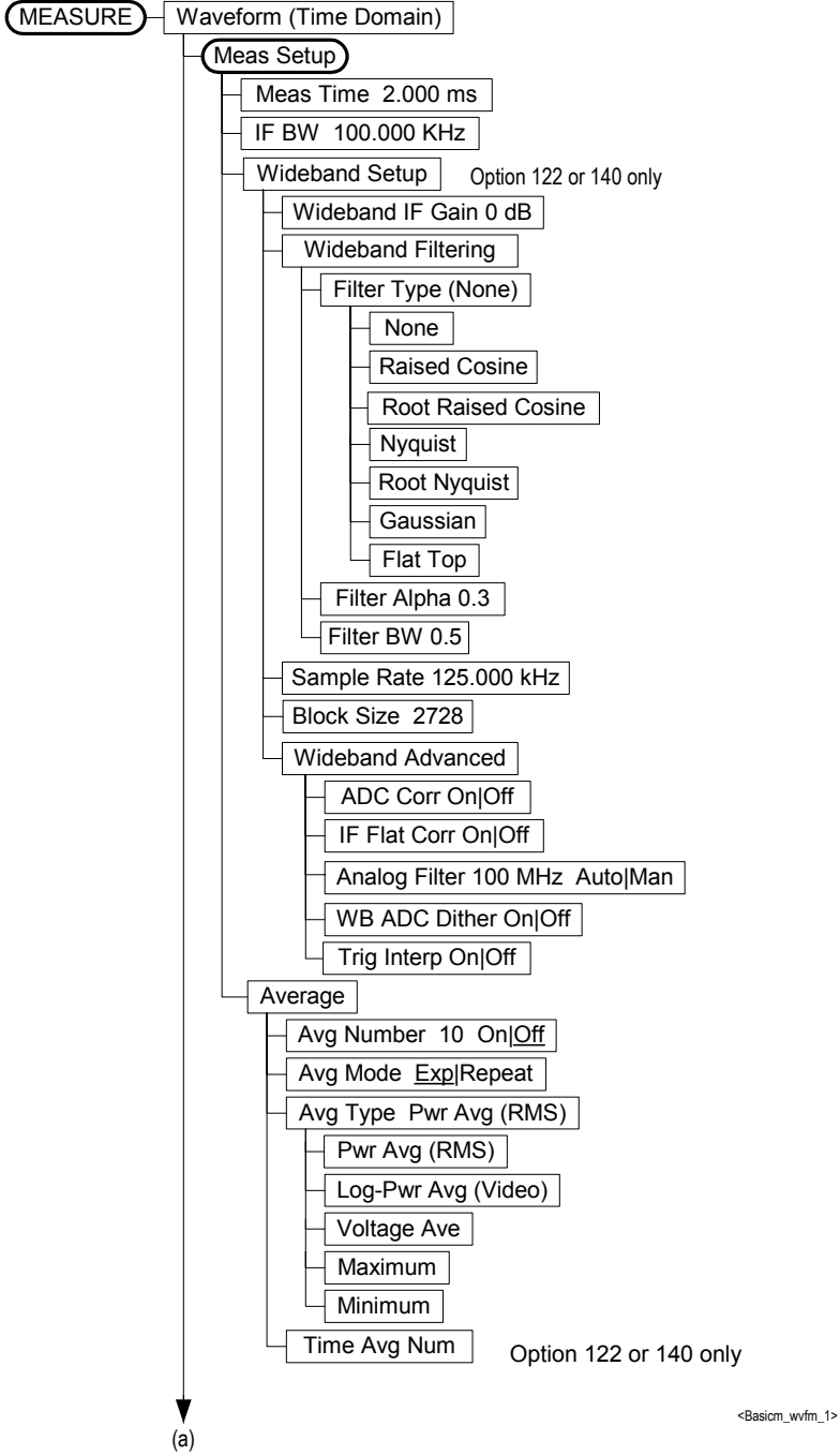
Figure 6-7 Waveform (Time Domain) Measurement Key Flow (1 of 3)
