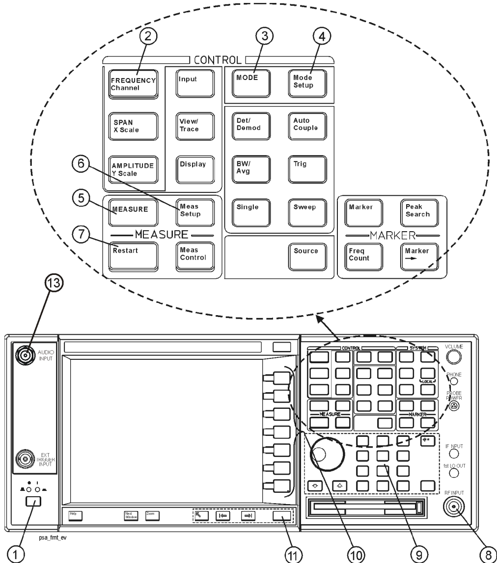
Figure 3-1 PSA Selected Front Panel Key Locations
